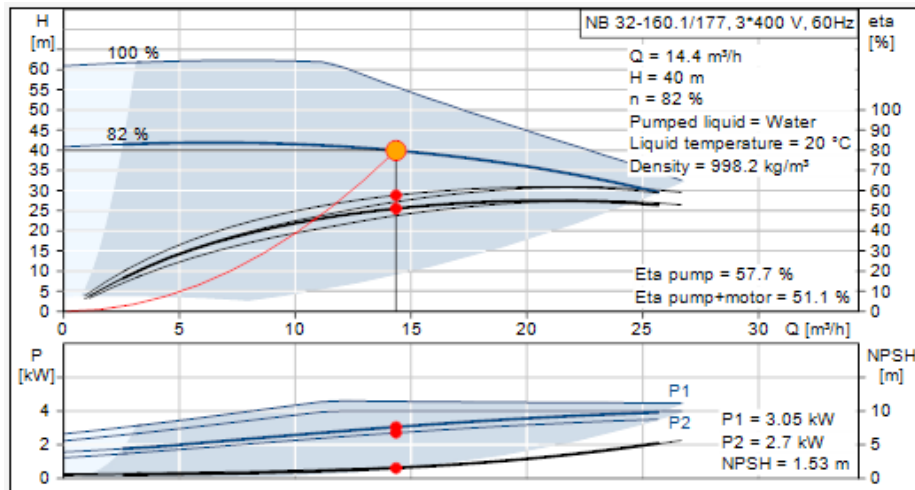
Figure 4.2.3: Proposed coil cooling pump
