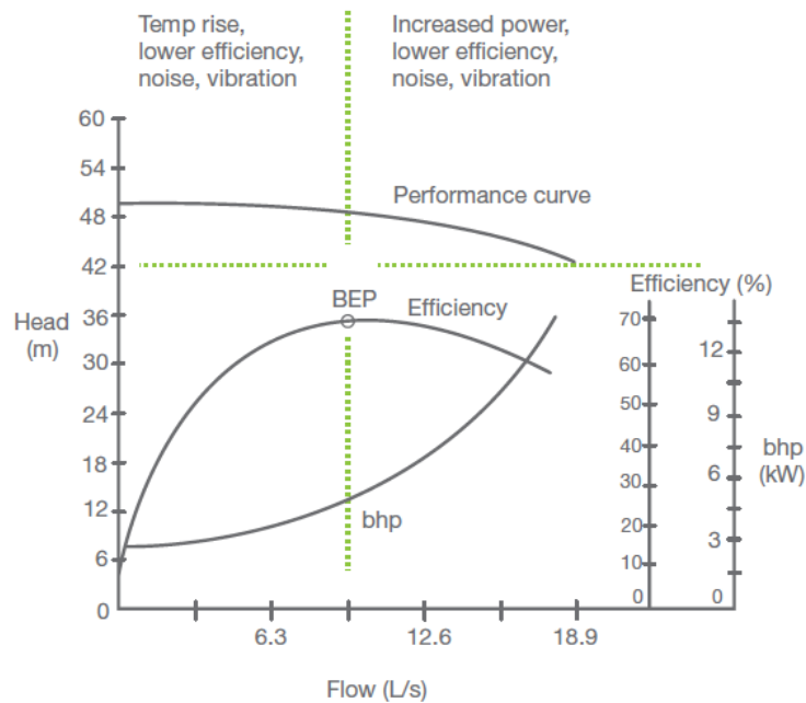
Figure 4.2.1: Pump operating point
