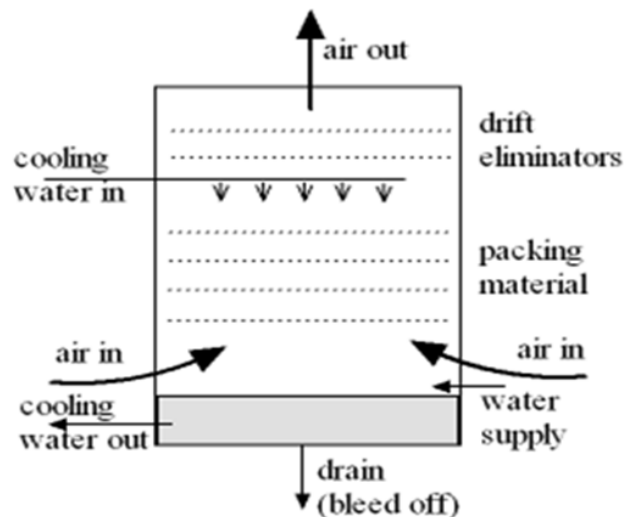
Figure 4.2.2b: Schematic view of cooling tower
