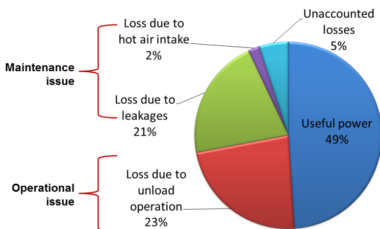
Figure 4.1.2c: Energy balance of air compressor
