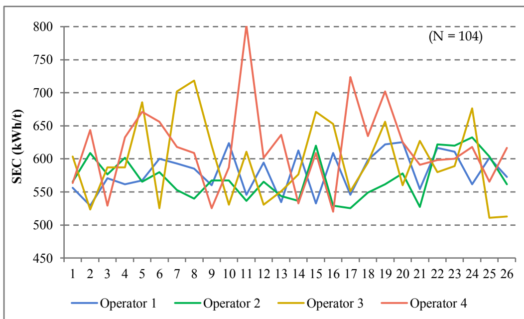
Figure 3.2.3i: Operator vs. SEC
