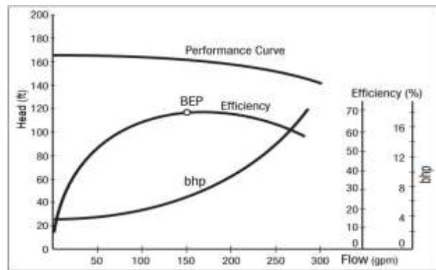
Best efficiency point in pump operation
