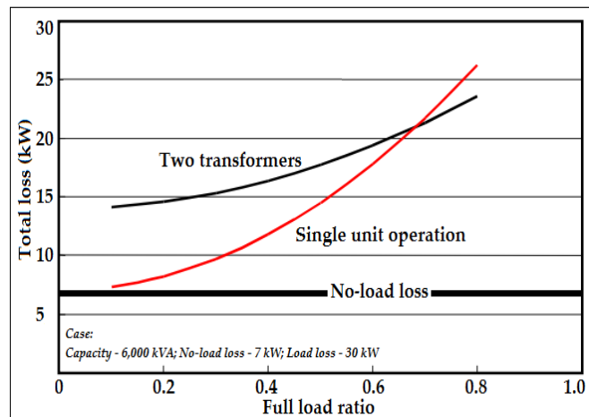
Parallel operation of transformers
